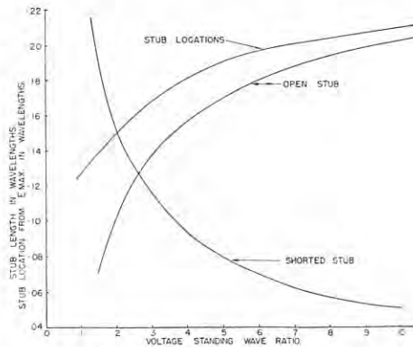
FIG 11 DETERMINATION OF STUB LENGTHS AND LOCATIONS IN IMPEDANCE MATCHING
