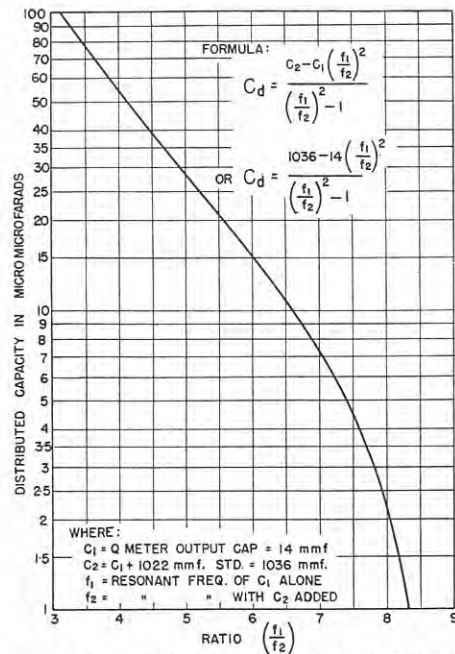
FIG. 3. - MEASUREMENT OF DIST. CAP. OF COIL
