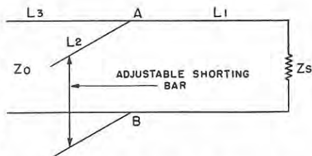
FIG 10—MATCHING WITH A STUB LINE
