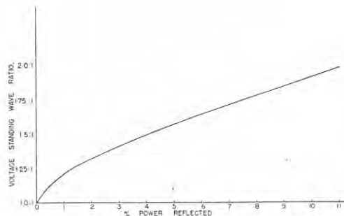
FIG 9 VOLTAGE STANDING WAVE RATIO VS REFLECTED POWER
