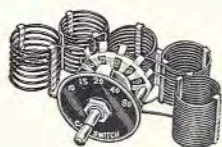
50 Watt Bank Switch Assembly
